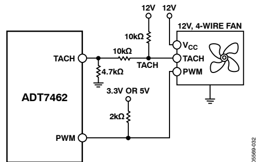
Figure 42. Driving a 4-Wire Fan
