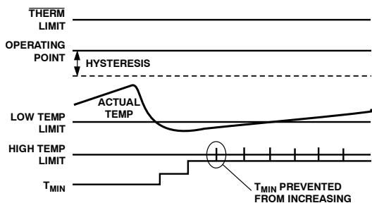
Figure 74. T MIN Adjustments Limited by High Temperature Limit
