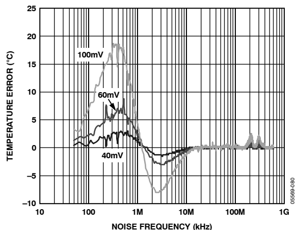
Figure 18. Remote Temperature Error vs. Common-Mode Noise Frequency
